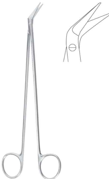
POTTS DE MARTEL 21,0 cm, 8 1 / 4 " 11-4548-21 24,0 cm, 9 1 / 2 " 11-4548-24
